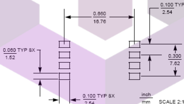
Figure 14. Small outline package footprint
