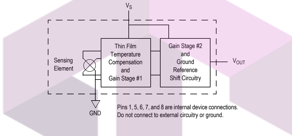
Figure 3. Integrated pressure sensor block diagram
