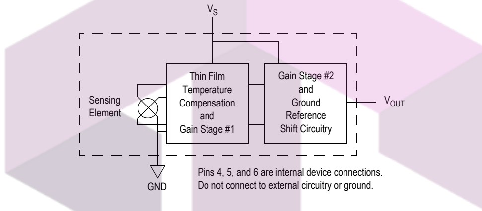
Figure 1. Integrated pressure sensor block diagram
